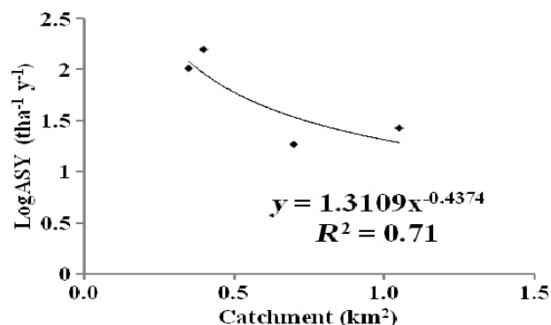
Fig. 5. Relationship between area-specific sediment yield and catchment area for study reservoirs.
