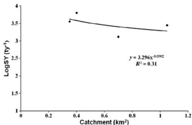
Fig. 4. Relationship between sediment yield and catchment area for study reservoirs.
