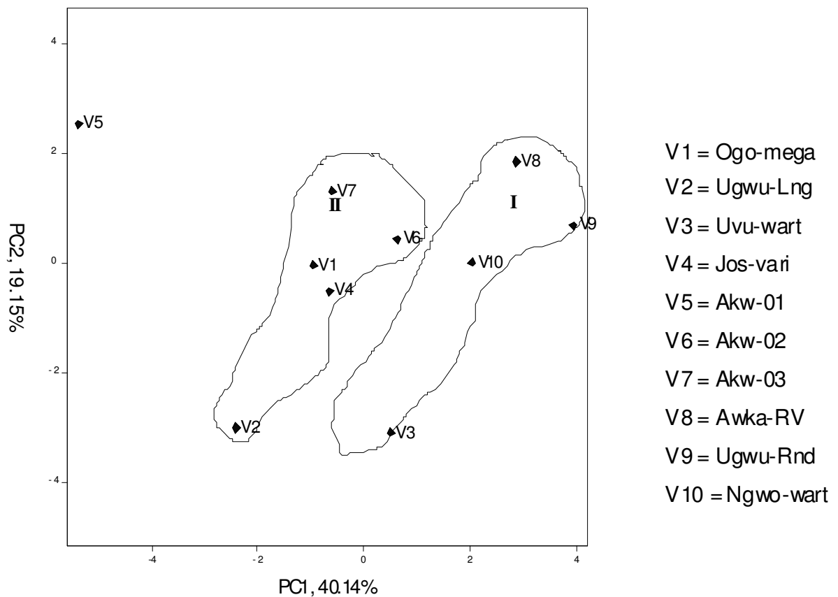
Figure 2. First and second principal component scores (PC1 and PC2) for the identification of Cucurbita accession performance on the 19 quantitative traits.
