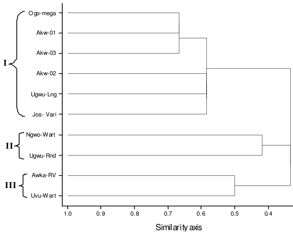
Figure 4. Dendrogram of 10 Cucurbita accessions based on qualitative characters.
