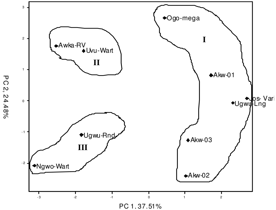
Figure 3. First and second principal component scores (PC1 and PC2) for the identification of Cucurbita accession performance on the 14 qualitative traits.
