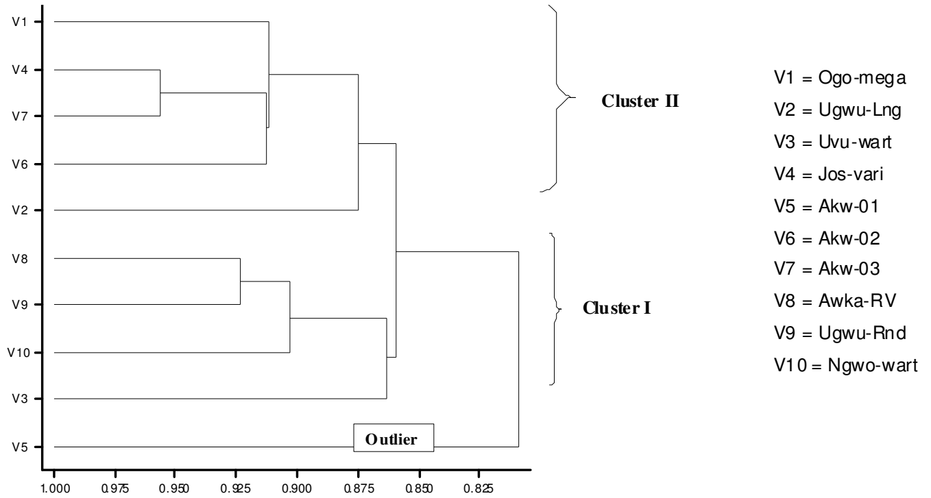
Figure 1. Dendrogram of 10 Cucurbita accessions based on quantitative characters.
